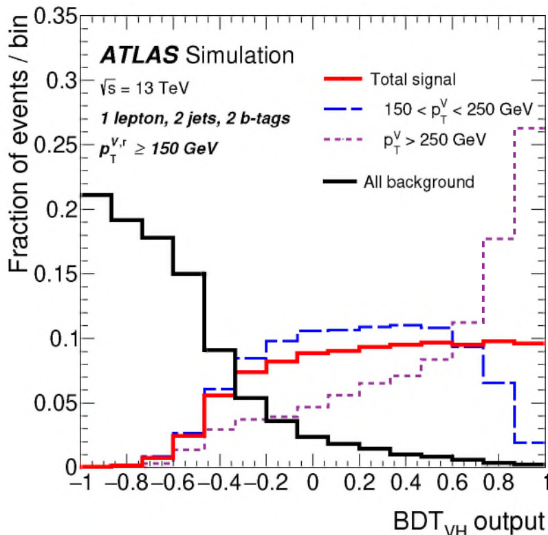
Figure 1. BDT_{VH} distributions for different p_T^V STXS regions in the 1-lepton, 2-jet reconstructed-event category. Only regions contributing at least 10% of the expected signal yield in the reconstructed-event category are displayed. The distributions of the total signal and background are also shown. The BDT_{VH} distributions are scaled to the same (unit) area to highlight the shape differences.
