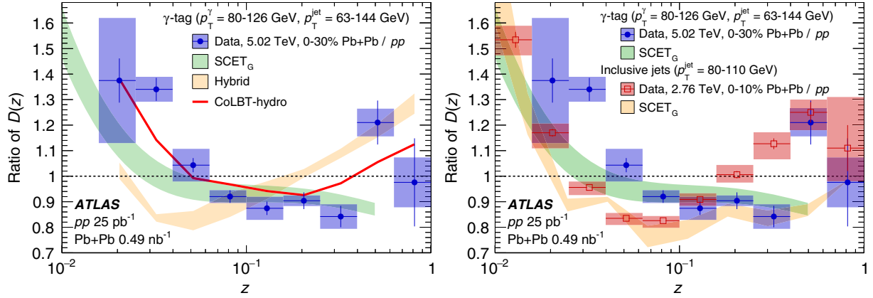
FIG. 3. Comparison of the ratio of \gamma -tagged fragmentation function D(z) in central Pb + Pb events to pp events with theoretical calculations (left). The mutual comparison between \gamma -tagged and inclusive jet D(z) ratios in data to each of these in the SCET G model is shown in the right panel. Shaded rectangles and vertical bars show the total systematic and statistical uncertainties, respectively, in the data.
