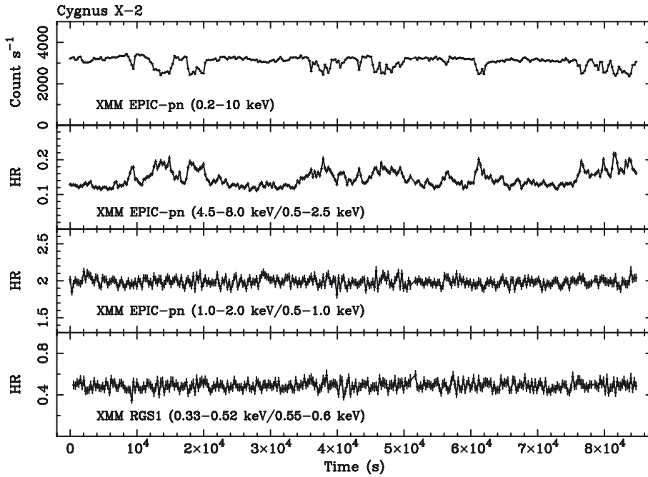
Fig. 2. Hardness ratios defined in several energy bands: upper middle panel: using wide EPIC-pn bands; lower middle band: using EPIC-pn bands below 2 keV; lower panel: using the RGS1 band. The upper panel gives the 0.2–10 keV EPIC-pn lightcurve for comparison.
