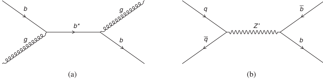
FIG. 1. Example of the leading-order Feynman diagram for production and decay of (a) b^* and (b) Z' into final states involving b quarks.
