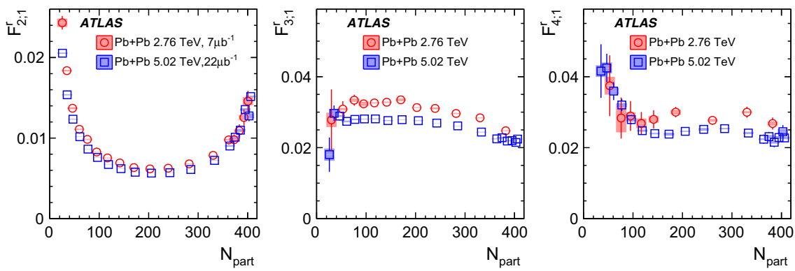
Fig. 11 Centrality dependence of F_{2,1}^r (left panel), F_{3,1}^r (middle panel) and F_{4,1}^r (right panel) for Pb+Pb at 2.76 TeV (circles) and 5.02 TeV (squares). The error bars and shaded boxes are statistical and system-
