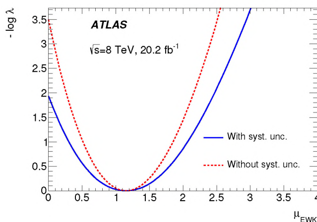
Figure 7. The profile of the negative log-likelihood ratio \lambda(\mu_{EWK}) of the signal strength \mu_{EWK} of the \zeta_{Z\gamma} template. The observed result is shown by the solid curve, while the dashed curve shows the results with only the statistical uncertainty included. The observed significance of the measurement is given by \sqrt{-2\log\lambda(0)} and equals 2.0\sigma in this case.
