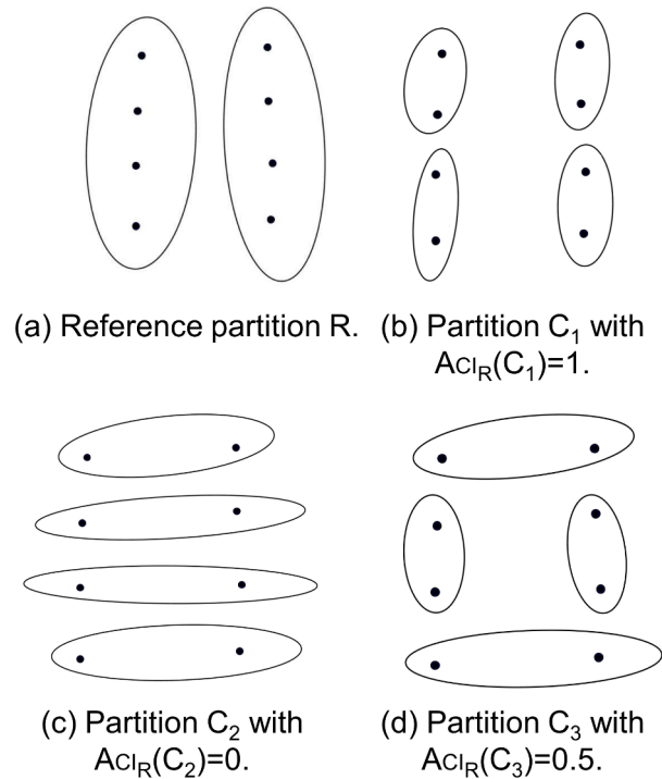
Figure 3. Illustration of the AcI. Partition C_1 fully reflects the reference, R ( ACI_R(C_1)=1 ). In contrast, partition C_2 is random with respect to the reference – the two results do not share any information ( ACI_R(C_2)=0 ). Partition C_3 is a combination of the two previous situations – half of the reference can be recovered from this clustering ( ACI_R(C_3)=0.5 ). doi:10.1371/journal.pone.0102069.g003
