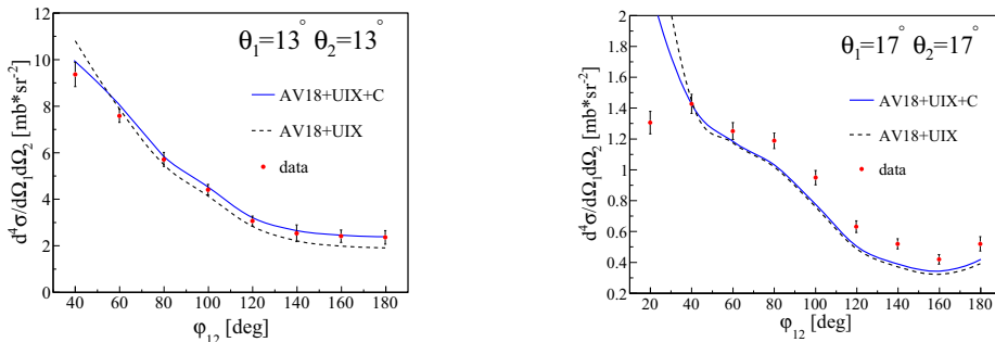
Figure 2. Differential, integrated over energy, cross-section values presented as a function of the relative azimuthal angle \varphi_{12} , for a given \theta_1, \theta_2 combination. The presented data were obtained at 130 MeV (left panel) and at 160 MeV (right panel) deuteron beam energies. The data are compared with the calculations indicated in the legend.
