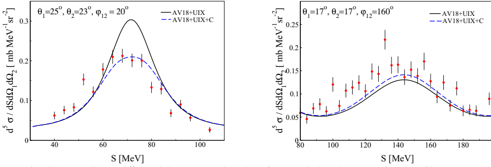
Figure 1. (Color online) Differential cross-section data for the dp breakup reaction at 160 MeV at two different kinematical configurations (specified in the panels). In the configuration presented on the left panel significant Coulomb force effects are observed. The data are compared to the AV18-based calculations and are described in the legend.
