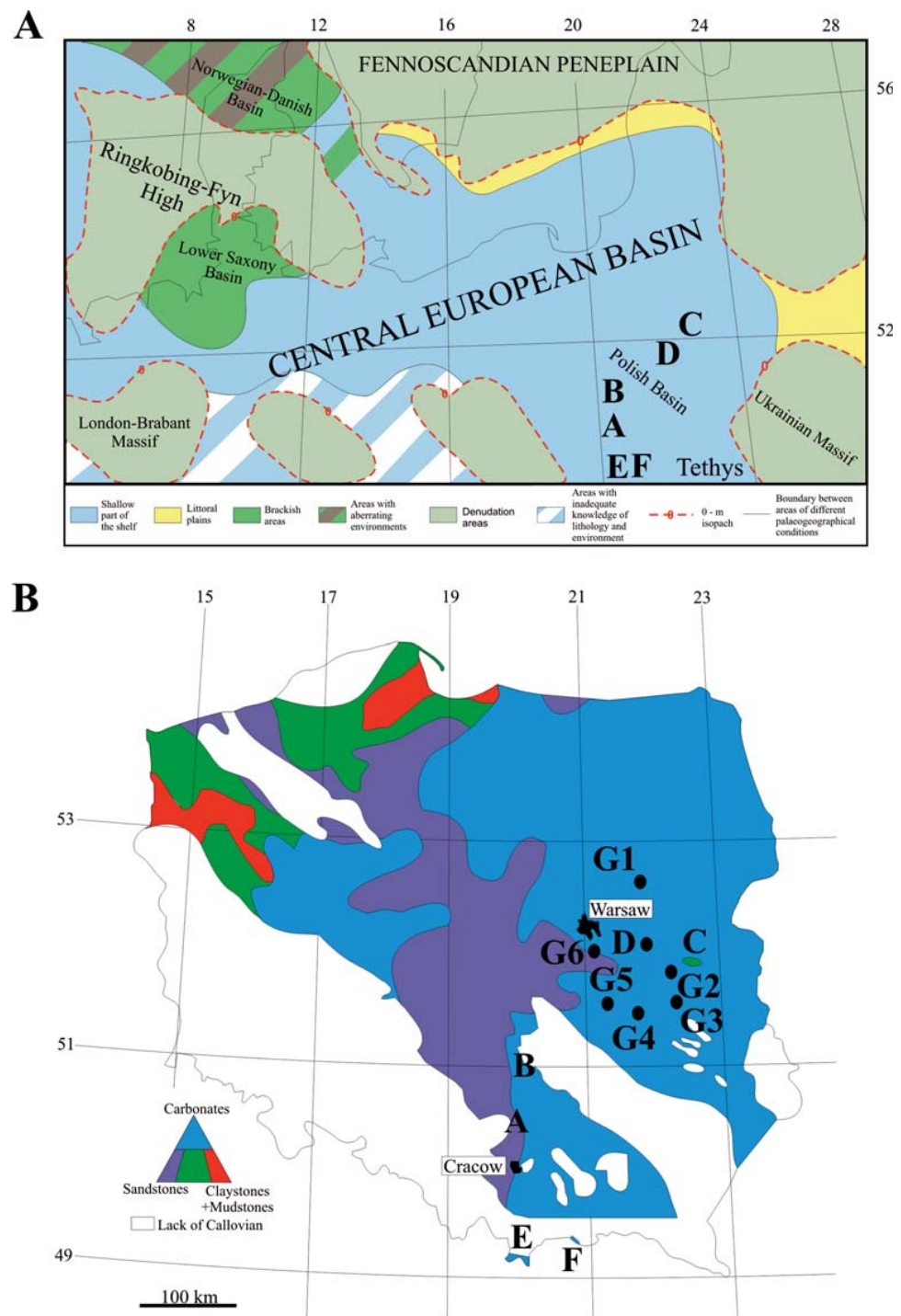
Figure 1 Location maps. (A) Palaeogeographic map of central Europe during the Middle Jurassic (modified after Šimkevičius, Ahlberg & Grigelis, 2003). (A) Bathonian and Callovian exposures of the southern part of the Polish Jura; (B) Bathonian and Callovian exposures of the southern margin of the Holy Cross Mountains; (continued on next page...)
