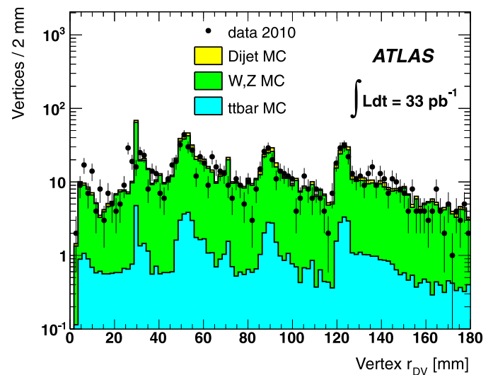
Fig. 5. Comparison of the m_{DV} (top), N_{DV}^{\text{trk}} (center), and r_{DV} (bottom) distributions of data and MC events in the control region m_{DV} < 10 GeV. Other than the material veto and the N_{DV}^{\text{trk}} \geq 4 and m_{DV} > 10 GeV requirements, all selection criteria are applied. In addition, the N_{DV}^{\text{trk}} and r_{DV} distributions include a veto on K_S^0 decays. The MC histograms are normalized to the integrated luminosity of the data, with the MC cross-section given by PYTHIA [11].
