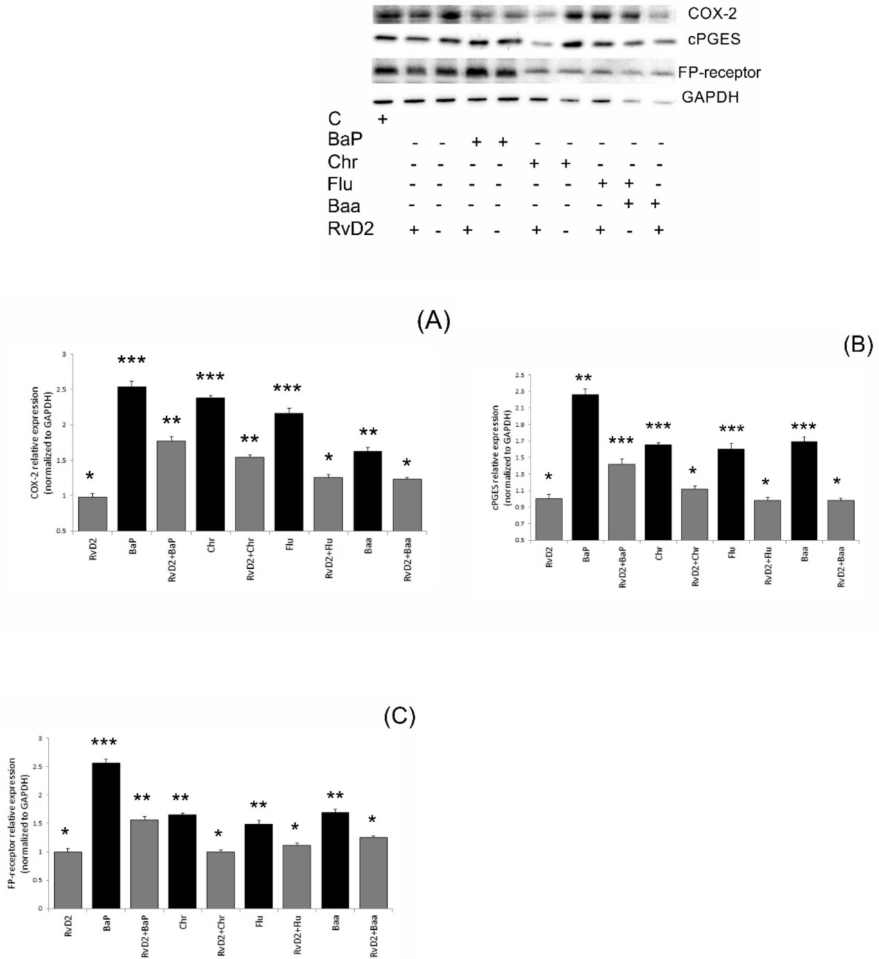
Fig. 1. Relative expression of COX-2 (A), cPGES (B) and FP-receptor (C) in RAW 264.7 cells treated with PAHs and incubated with RvD2. Asterisks denotes statistically significant differences at P<0.05.
