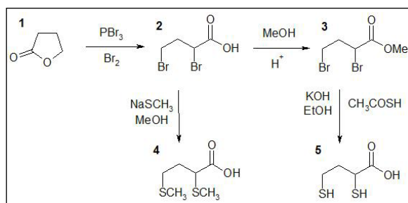
Fig.1. Synthesis of lipoic acid derivatives; (1) \gamma -butyrolactone; (2) 2,4-dibromobutanoic acid [BMTBA]; (3) methyl 2,4-dibromobutanoate; (4) 2,4-bis(methylthio)-butanoic acid [BMTBA]; (5) 2,4-dimercaptobutanoic acid (tetranor-dihydroliipoic acid, tetranor-DHLA)
