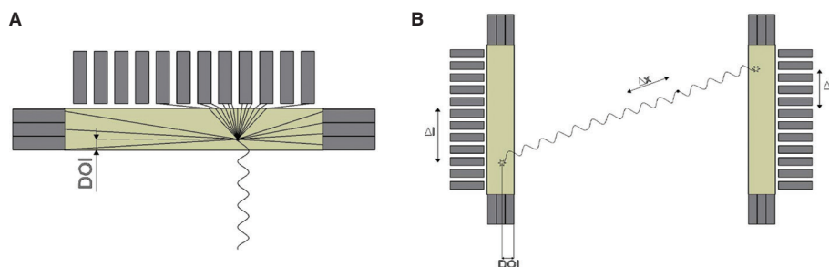
Figure 3. A. Schematic view of the cross section of a single detection plate for the MATRIX-PET. B. The hit position versus the center of the scintillator ( \Delta l ) is determined based on time difference measured on both sides of the scintillator plate and independently based on the amplitude distributions of signals in the matrix of photomultipliers surrounding the plate. A position ( \Delta x ) along the LOR is determined from time difference measured between two plates
