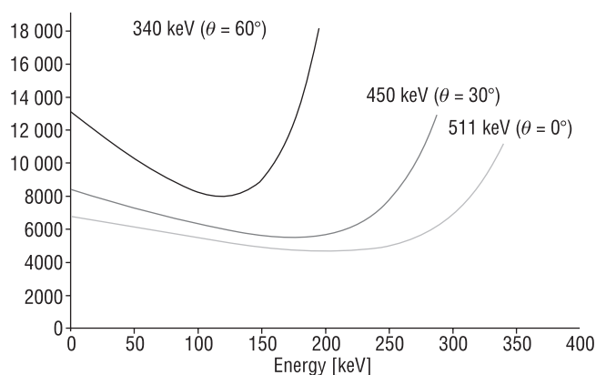
Figure 1. Energy distribution of electrons scattered in the Compton effect by gamma quanta with an energy shown in the plot [9]. The distributions were made without taking into account the energy resolution, which for plastic detectors is about 18% (compared to energy resolution of about 12% for LSO blocks [3])
