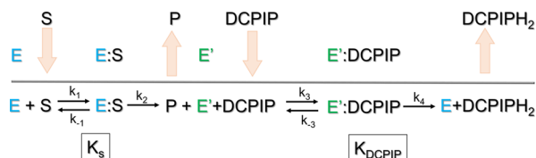
Figure 4. Schematic representation of the nonsequential Ping-Pong bi-bi mechanism. 64–66 K_S and K_{DCPIP} are dissociation constants of complexes E:S and E':DCPIP, respectively. k_2 and k_4 represent k_{cat} for RHR and OHR, respectively.
