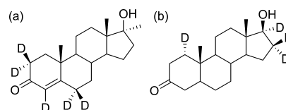
Figure 3. Deuterium-labeled 2,2,4,6,6- d 5 -17-MT (a) and 1,1,6,16,17- d 5 -DHT (b) used in the calculations and experiments.
