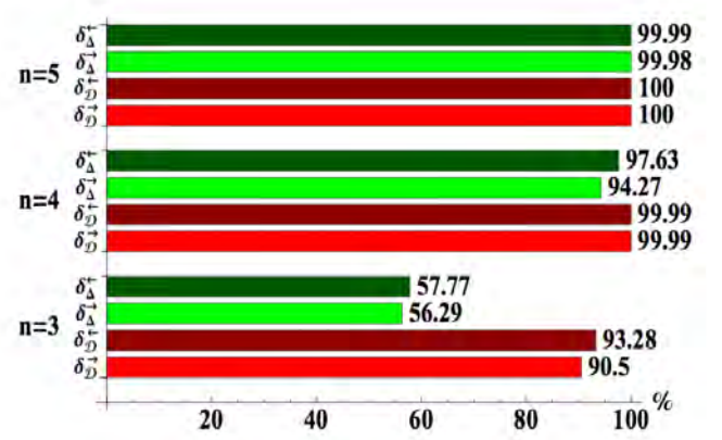
FIG. 14: Percentages of Haar uniformly generated states satisfying the monogamy relations for quantum discord and work deficit. The number of parties is denoted as “n” in the diagram. The monogamy scores for \mathcal{D}^+ , \mathcal{D}^- , \mathcal{W}\mathcal{D}^+ , and \mathcal{W}\mathcal{D}^- are respectively denoted in the diagram by \delta_{\mathcal{D}}^+ , \delta_{\mathcal{D}}^- , \delta_{\mathcal{D}}^+ , and \delta_{\mathcal{D}}^- . [Reprinted from Ref. [735] with permission. Copyright 2015 American Physical Society.]
