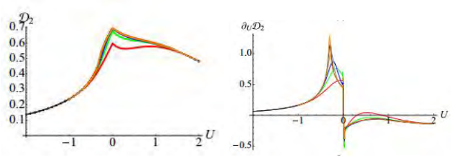
FIG. 8: (Left panel) Néel AFM - Haldane transition by using symmetric QD between nearest-neighbor sites, and (right panel) its derivative for the reduced state of the two central spins of an open-ended chain, described by the Hamiltonian in Eq. (74) of lengths 8 (red), 16 (green), 32 (blue), 64 (gray), 128 (black), and 256 (orange) going from bottom to top. The symmetric QD in the vertical axis is denoted by \mathcal{D}_2 in the figure while it is \mathcal{D}_{sym} in the text. The vertical axes are in bits while the horizontal ones are dimensionless. [Reprinted from Ref. [499] with permission. Copyright 2015 American Physical Society.]
