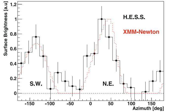
Fig. 6. Azimuthal profile obtained from HESS data and XMM-Newton data in the 2–4.5 keV energy band and smoothed to HESS PSF, restricted to radii 0.12^\circ \leq r \leq 0.36^\circ from the centre of the SNR. Azimuth 0^\circ corresponds to East, 90^\circ corresponds to North, 180^\circ to West and -90^\circ to South.
