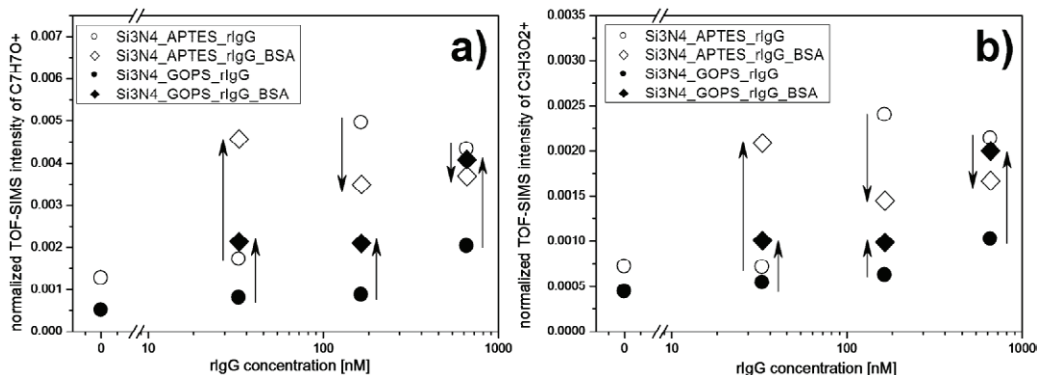
Fig. 3. Intensity of secondary ions characteristic for proteins \text{C}_7\text{H}_7\text{O}^+ (left, m/z = 107.05 , from Tyr) and \text{C}_3\text{H}_3\text{O}_2^+ (right, m/z = 71.01 , from Ser) indicates higher rIgG adsorption to \text{Si}_3\text{N}_4 surfaces modified with APTES (open circles) rather than GOPS (solid circles) and different behavior (indicated with arrows) to subsequent blocking with BSA (diamonds).
