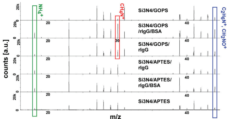
Fig. 2. Representative positive ion TOF-SIMS spectra of the \text{Si}_3\text{N}_4 surfaces, modified with APTES and GOPS, respectively, prior to and after immobilization of rIgG (660 nM) and blocking with BSA. Signals characteristic for proteins are marked with rectangles.
