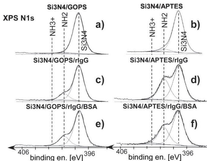
Fig. 1. High resolution N1s core-level XPS spectra of two series of \text{Si}_3\text{N}_4 surfaces modified with GOPS (a, c, e) and APTES (b, d, f). Distinct contributions from \text{Si}_3\text{N}_4 and amine ( \text{NH}_2 and protonated \text{NH}_3^+ ) groups are visible, characteristic for silanized substrates (a, b) and protein overlayers formed due to coating with rIgG (660 nM) (c, d) and blocking with BSA (e, f).
