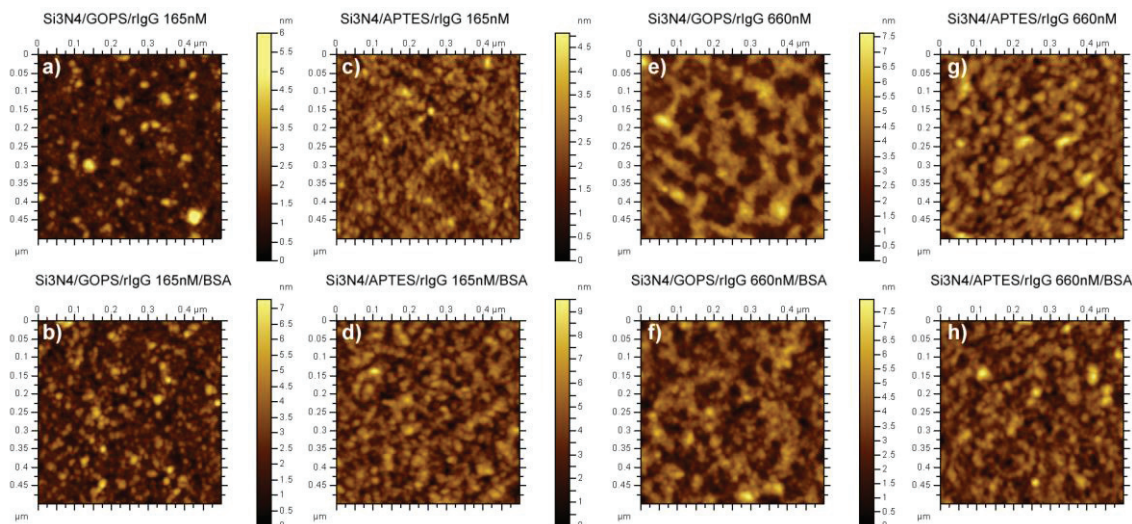
Fig. 4: AFM images of \text{Si}_3\text{N}_4 surfaces after adsorption of rIgG from 165 nM (a, c) and 660 nM (e, g) solutions, followed by subsequent blocking with BSA (b, d, f, h). The blocking resulted in visibly increased protein coverage for rIgG coated surfaces modified with GOPS (a-b and e-f) rather than for those modified with APTES (c-d and g-h).
