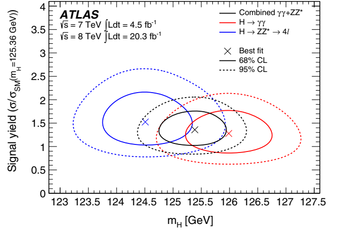
FIG. 9 (color online). Likelihood contours -2\ln\Lambda(S, m_H) as a function of the normalized signal yield S = \sigma/\sigma_{\text{SM}}(m_H = 125.36 \text{ GeV}) and m_H for the H \rightarrow \gamma\gamma and H \rightarrow ZZ^* \rightarrow 4\ell channels and their combination, including all systematic uncertainties. For the combined contour, a common normalized signal yield S is used. The markers indicate the maximum likelihood estimates in the corresponding channels.
