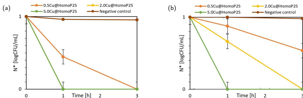
Figure 4. The influence of the copper-modified HomoP25 and RMF with the frequency of 25 Hz on the growth of E. coli (a) and S. epidermidis (b).
