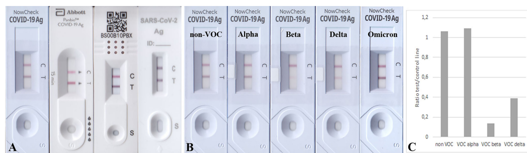
FIGURE 2 (A) RATs (BioNote, Abbott, Boson, and TIB) loaded with 100 ng recombinant N-protein of the non-VOC strain. All used RATs detected this amount of protein. (B) The exact amount of protein produced a comparable test line in the case of Alpha and Omicron, but the test lines using protein from Beta and Delta appeared much weaker. (C) Densitometric analysis of RATs shown in (B). The N protein from all variants was detected, but for Beta and Delta, the sensitivity seems much lower.
