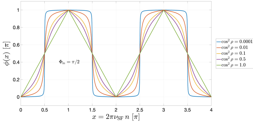
FIG. 7. Phase motion of the horizontal polarization envelope for \Phi_{\text{in}} = \pi/2 as predicted by Eq. (45). In the limit of \cos \rho \rightarrow 0 , the phase motion evolves into the phase jumps and the central bumps at x = \pi and 3\pi exhibit a rectangular shape.
