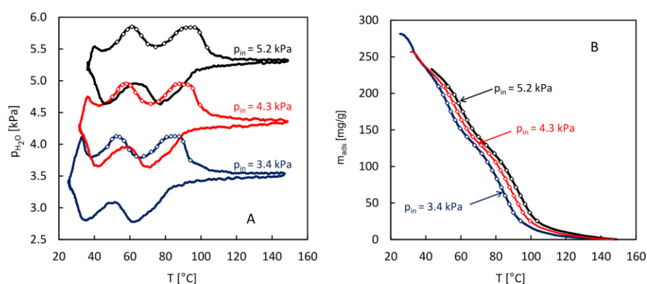
Figure 4. The QE-TPDA profiles (A) of water observed in the new experimental system for MIL-96 at a heating/cooling rate of 2 °C/min at different inlet partial pressures, and the corresponding integral desorption curves (B). The points indicate data found for the preset adsorbed amount values (from 25.5 to 209.5 mg/g, with 11.5 mg/g interval). Experimental details: sample mass m = 5.5 mg, carrier gas (N 2 ) flowrate F = 8.0 cm 3 /min.
