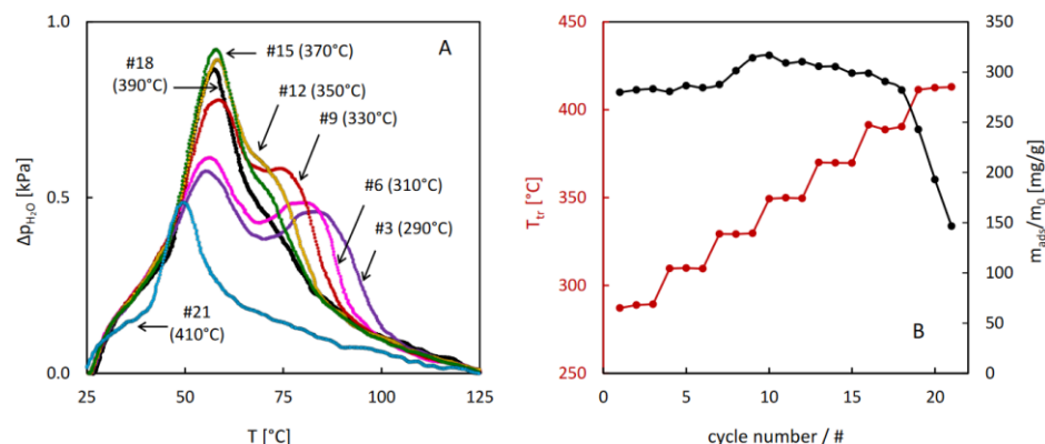
Figure 7. Results of the hydrothermal stability test for MIL-96: selected QE-TPD profiles corresponding to the last cycle in the 3-cycle sequences (A) and evolution of the hydrothermal treatment temperature and sorption capacity with the cycle number (B). Experimental details: heating rate \beta = 2^\circ\text{C}/\text{min} , inlet partial pressure of water p_{in} = 2.8\text{ kPa} , sample mass m = 3.0\text{ mg} , carrier gas ( \text{N}_2 ) flowrate F = 8.0\text{ cm}^3/\text{min} .
