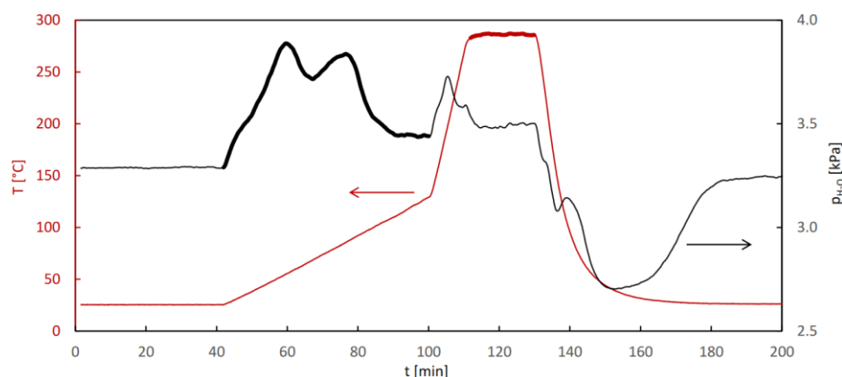
Figure 6. Illustration of the principle of the hydrothermal stability test: the evolution of the sample temperature and the detector signal during a single desorption–adsorption cycle. This example corresponds to the first cycle recorded for MIL-96 (see Figure 7). The diagnostic segment and the hydrothermal treatment segment are indicated by thick black and dark red lines, respectively.
