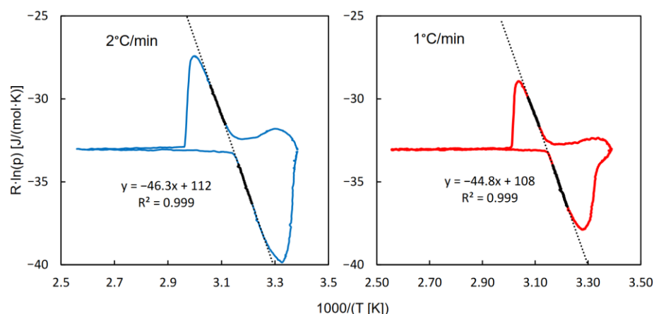
Figure 2. The QE-TPDA profiles from Figure 1B transformed according to the van't Hoff equation. The formulae in the insets indicate the values of the adsorption enthalpy and entropy and correlation coefficients obtained by linear regression of overlapping fragments of the profiles.
