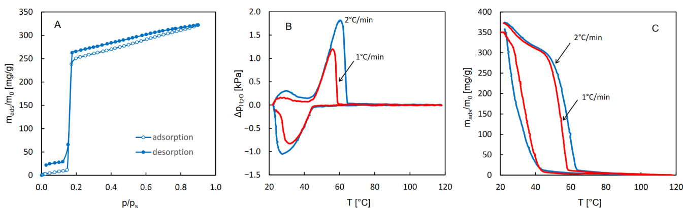
Figure 1. The isotherms of water adsorption and desorption measured at 25 °C (A) and QE-TPDA profiles (B) of water observed for CAU-10, as well as the integral adsorption and desorption curves (C), based on the thermodesorption profiles. Experimental details of QE-TPDA: inlet partial pressure of water p_{\text{in}} = 1.9 kPa, sample mass m = 3.3 mg, carrier gas (He) flowrate F = 7.2 cm 3 /min.
