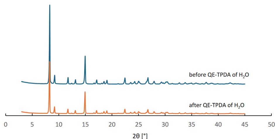
Figure 10. Powder XRD patterns of CAU-10 samples before and after the QE-TPDA of H 2 O measurements.
