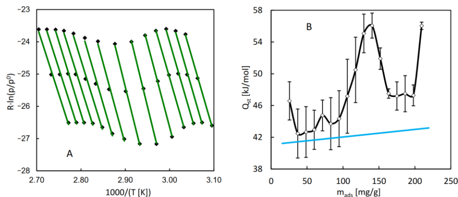
Figure 5. (A) The transformed adsorption isosteres of water on MIL-96 calculated from data indicated as points in Figure 4. (B) Isosteric adsorption heat of water on MIL-96 obtained from analysis of the adsorption isosteres. The blue line indicates the values of the condensation heat of water, corresponding to the average temperatures of particular isosteres.
