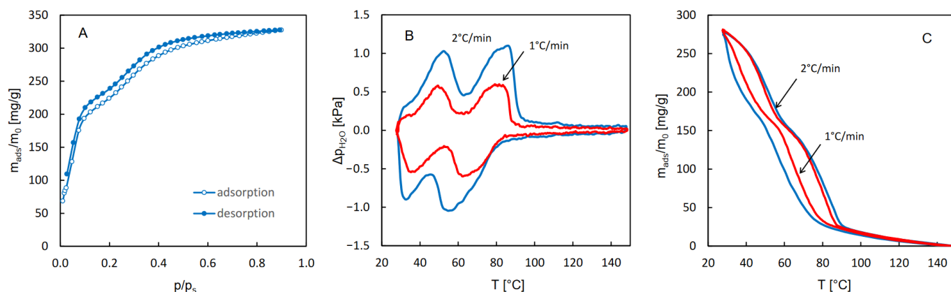
Figure 3. The isotherms of water adsorption and desorption (A) and QE-TPDA profiles (B) of water observed for MIL-96, as well as the integral adsorption and desorption curves (C), based on the QE-TPDA profiles from B. Experimental details of QE-TPDA: inlet partial pressure of water p_{\text{in}} = 2.4 kPa, sample mass m = 5.7 mg, carrier gas (He) flowrate F = 7.2 \text{cm}^3/\text{min} .
